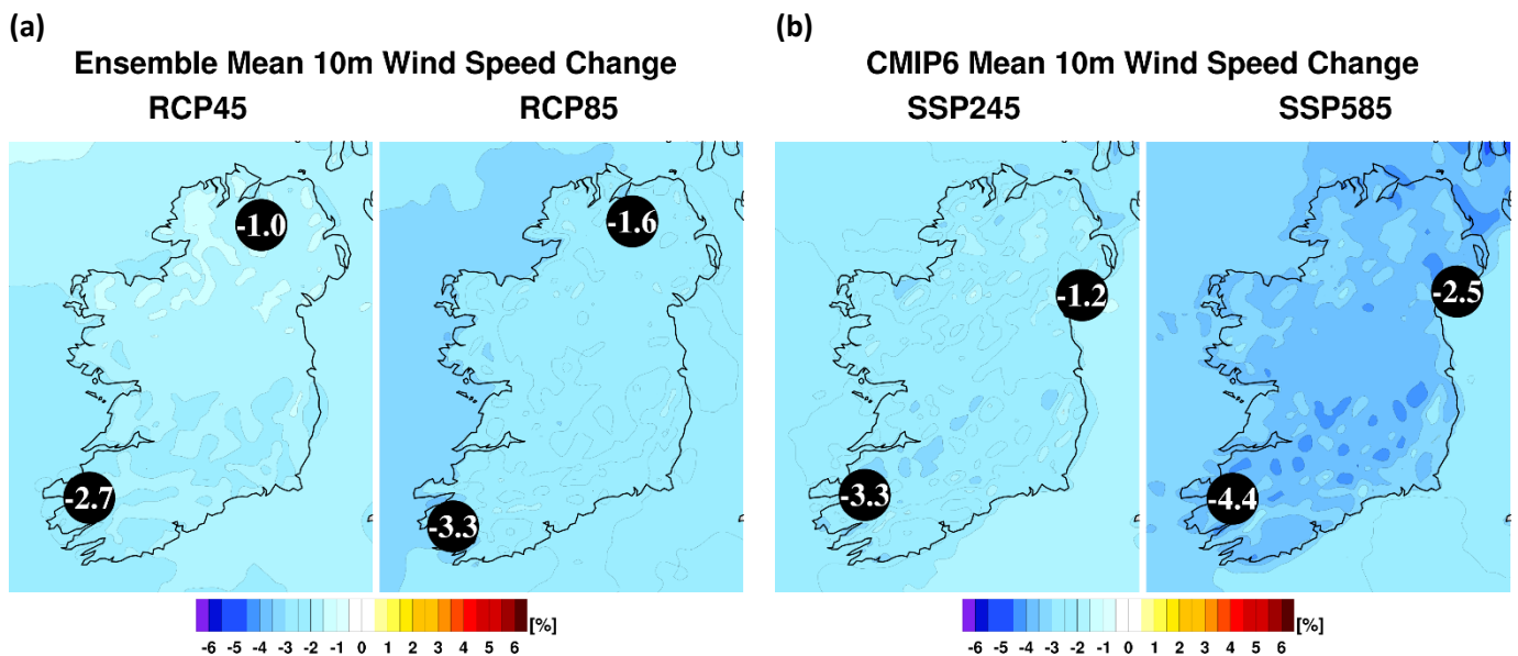
Figure 13. Projected change (%) in mid-century 10m wind speed for (a) CMIP5 and (b) CMIP6. In each case, the future period 2041–2060 is compared with the past period 1981–2000.
