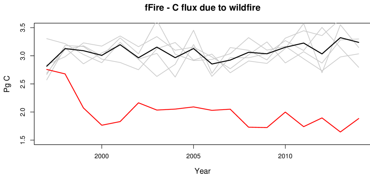
Figure 1: Carbon flux due to wildfire: estimations from GFED4s, compared to first year forecasts from the offline version of LPJG (with the GlobFIRM model) forced by 5 members of the DCPD forecasts done by BSC.
