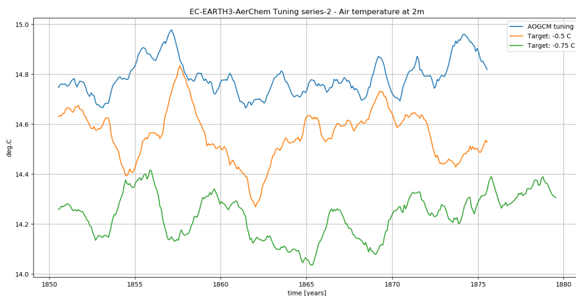
Figure 1. Global mean surface air temperature in the three EC-Earth3-AerChem pre-industrial spinup runs, which are currently running. The three model configurations differ only in the values of three atmospheric tuning parameters: the blue curve is produced using the standard settings from EC-Earth3, while the orange and green curves are obtained after re-tuning the model, where the target was to cool the model by about 0.5 K and 0.75 K, respectively, compared to the configuration with standard settings. Note that all simulations were started from the same initial state obtained with EC-Earth3; the first 120 years of the simulations are not shown.
