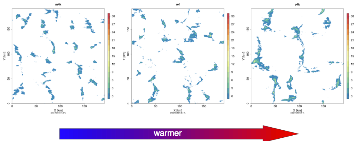
Figure 2. Snapshots of simulated precipitation intensity for the reference simulation (middle) and 4 degrees cooler and warmer conditions, left and right panel respectively. The snapshot is taken around hour 5 after the onset of precipitation (see Figure 1).
