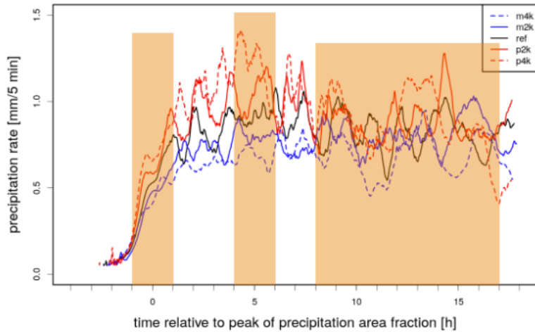
Figure 1. Time evolution of rainfall intensity in the 5 experiments, from coldest (blue dashed) to warmest runs (red dashed lines)
