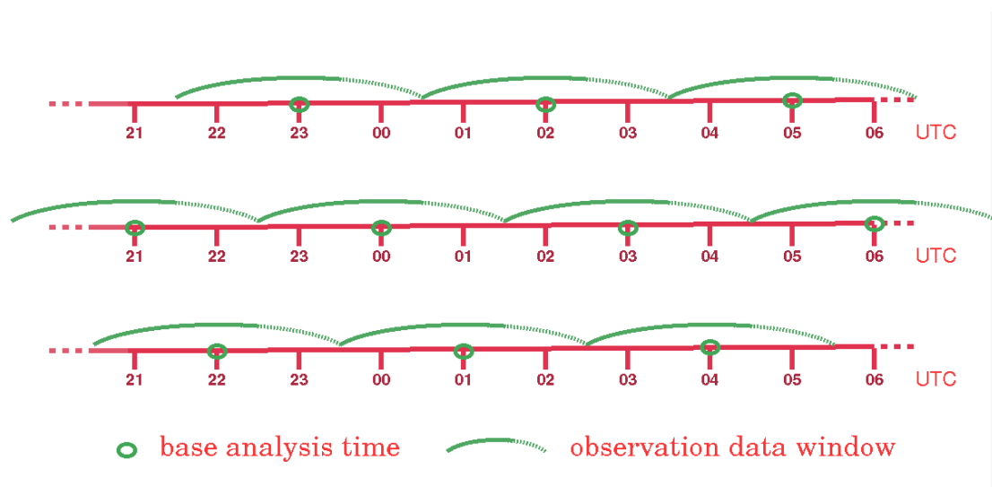
Fig. 1: Overlapping time window strategy used in the present COMECS ensemble. Hourly analysis is enabled in DMI's COMECS ensemble system through the use of 3 parallel suites, each using a 3-hourly data assimilation cycling but with a base time which is consecutively shifted by 1h between the three members. This way, every hour a 3D-VAR analysis is launched with a 3h observation window. As the three consecutive assimilation cycles are mutually independent, the repeated use in observations in overlapping time windows between the three consecutive suites is not a problem, as it would be for the traditional deterministic 3D-Var approach. In the envisaged future nowcasting ensemble system, the three consecutively hourly shifted suites with a 3h observation window each will be replaced by a set of 6 suites, shifted in base time by 10m between consecutive members, and using a 1h observation window. This system is aimed to assimilate rapidly delivered observations within a cutoff time of ~15m: mainly radar, surface observations and aircraft data.
