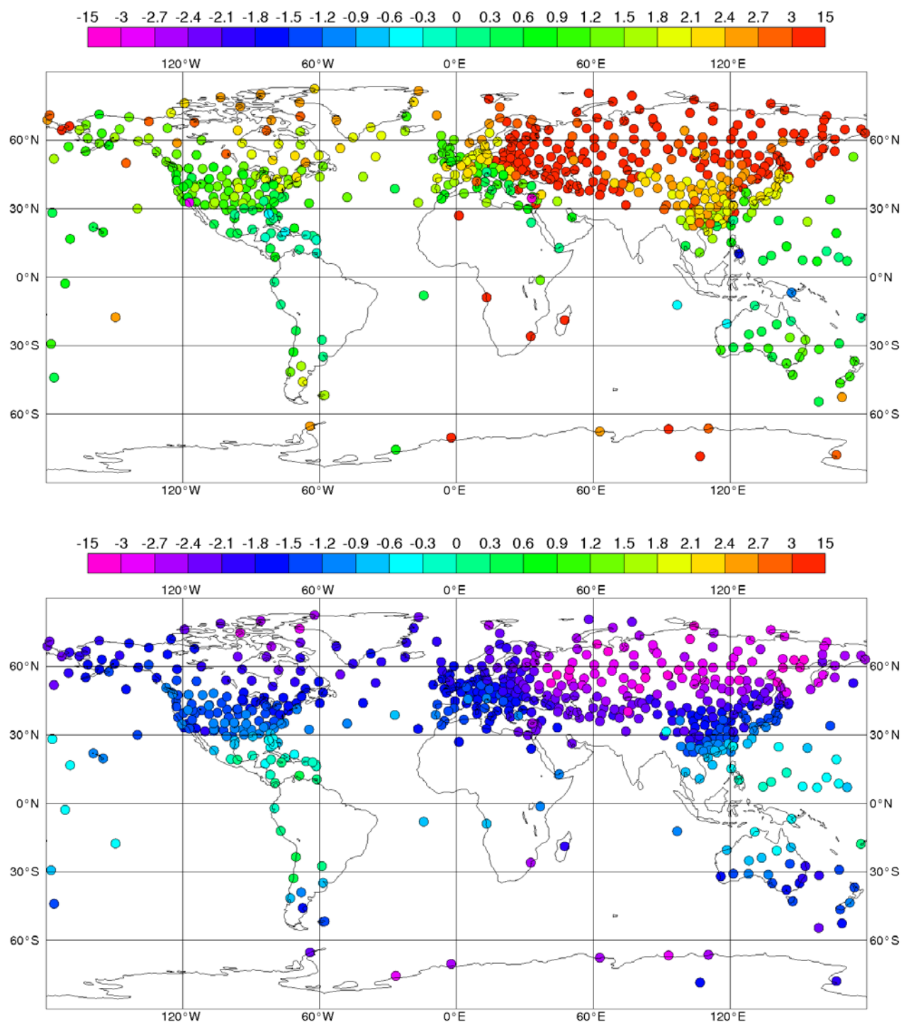
Fig. 1: obs-CERA20C (upper panel) and CERA20C-ERApreSAT temperature differences at the 300 hPa level averaged over 1958-1959, at least 18 months of data had to be available.
