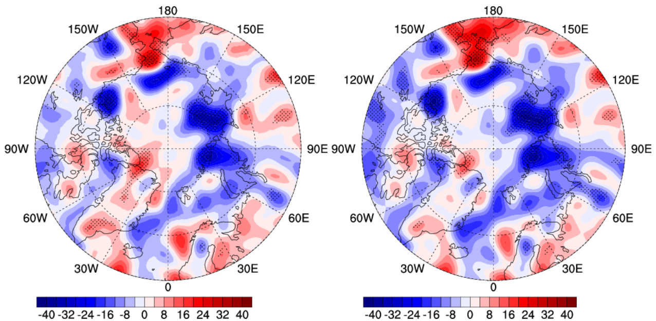
Fig. 5: Left panel: net surface energy flux (positive downward, units \text{Wm}^{-2}\text{decade}^{-1} ) trends 2000-2015 for month October, estimated indirectly as residual from CERES RadTOA fluxes and atmospheric energy flux convergence and storage. Right panel shows trends of atmospheric energy flux convergence.
