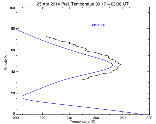
Fig. 2: Measured temperature profile
