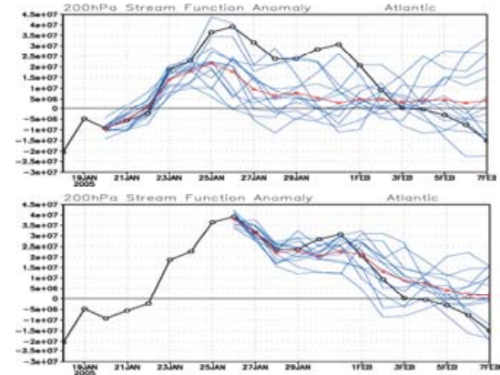
Fig. 4 Time series of area (60W-2.5E, 54N-60N) averaged stream function anomalies at 200hPa h from 18 th January to 7 th February 2005 for (black) observation, (red) ensemble mean, and (blue) each member. Unit is \text{m}^2/\text{s} . Upper panel is for prediction from 20 th January, and lower panel is for prediction from 26 th January 2005.
