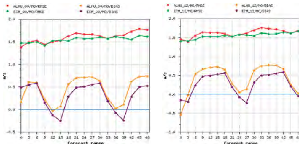
Fig.8 Comparison of BIAS and RMSE values for ECMWF and ALADIN wind speed forecasts over Hungary. Generally speaking the RMSE and BIAS errors are slightly smaller for the ECMWF model.
