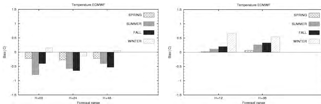
Fig. 8 Bias of 2m temperature over Portugal as function of forecast range, for summer, spring, fall and winter seasons for 12 UTC (left) and for 00 UTC (right).
