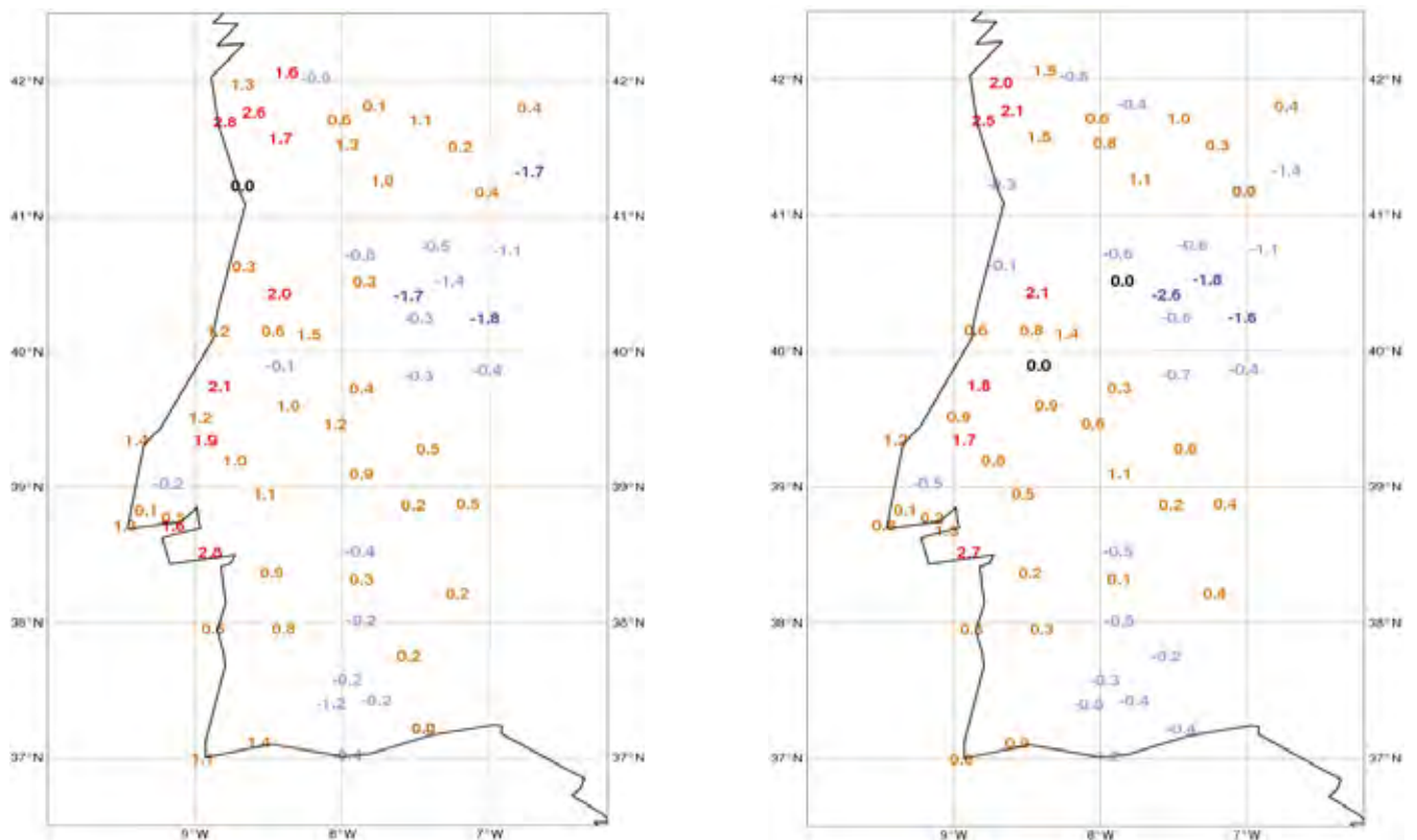
Fig. 6 Spatial distribution of 10m wind speed bias over Portugal, for H+24 (valid at 12 UTC), for fall (left) and spring (right) seasons. Positive values are in red (≥ 1.5 m s -1 ) and orange (< 1.5 m s -1 ). Negative values are in blue (< -1.5 m s -1 ) and cyan (≥ -1.5 m s -1 ).
