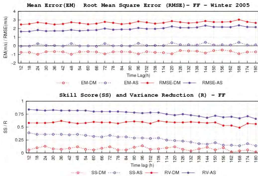
Fig. 14 Mean error (BIAS) and Root mean square error (RMSE) for Wind Speed (FF) (upper panel) and Variance Reduction and MSE_SS (lower panel), averaged over 168 stations. Winter 2005. (Red: DMO, Blue: MOS).
