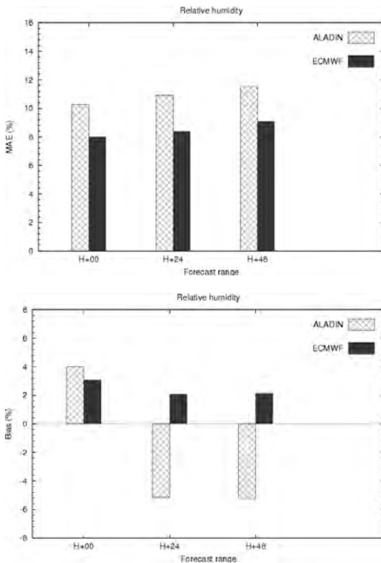
Fig. 15 MAE (top) and bias (bottom) of 2m relative humidity over Portugal as function of forecast range, for ECMWF and ALADIN models, for the autumn season.
