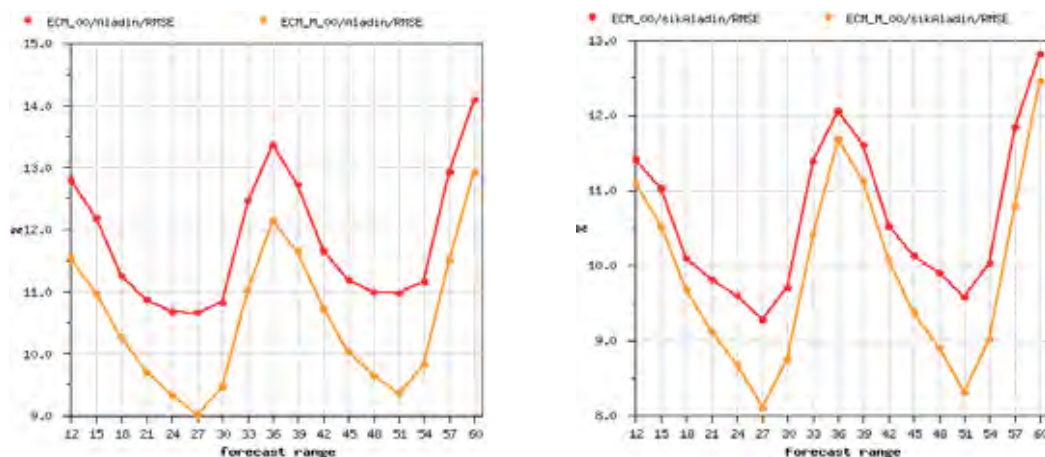
Fig. 14 RMSE error of the relative humidity forecasts before (red) and after (yellow) post-processing for an entire European area considering all the SYNOP stations (left panel), and only for the flat (<500 m) stations (right panel). The differences are not too big, but still noticeable regarding the fact that there are much less mountainous stations (>500 m), than flat ones.
