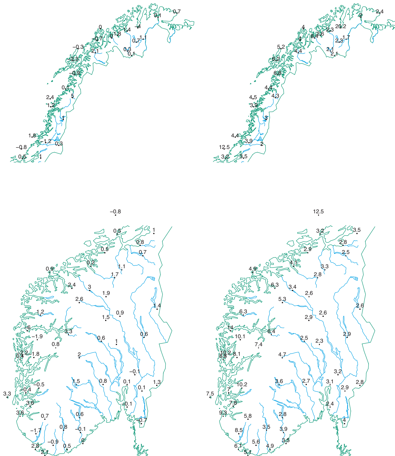
Fig. 2 Mean errors (left) and standard deviation of errors (right) of ECMWF 12+42 daily accumulated precipitation forecasts.
