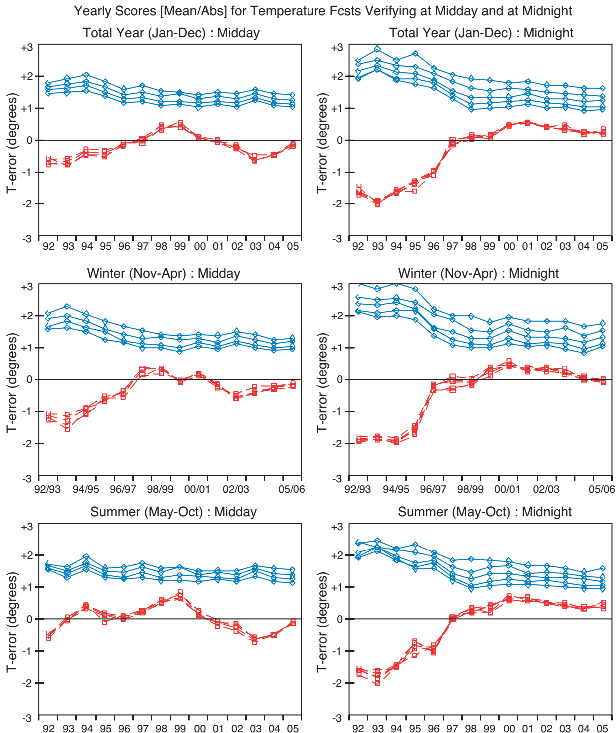
Fig. 6 Mean seasonal and yearly scores for ECMWF forecasts of 2-metre Temperature averaged over 6 stations. The blue lines indicate the error [mean absolute error], the red lines the bias [mean error]. Note that in 1992 the bias was much larger for the forecasts verifying at midnight rather than at midday but this effect became much less in later years [red lines]. Similarly, the error was greater, in 1992, for the midnight runs but gradually, over time, the difference became less [blue lines]. The errors for the various forecast lengths can be distinguished from the graphs: in all cases the top blue line corresponds to the longest forecast, the bottom blue line to the shortest.
