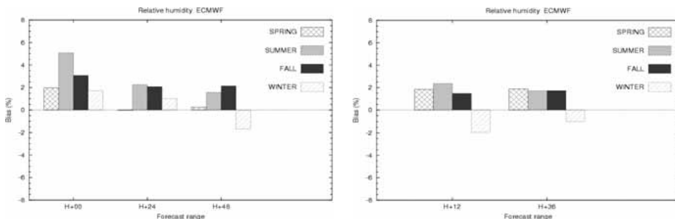
Fig. 10 Bias of 2m relative humidity over Portugal as function of forecast range, for summer, spring, fall and winter seasons for 12 UTC (left) and for 00 UTC (right).
