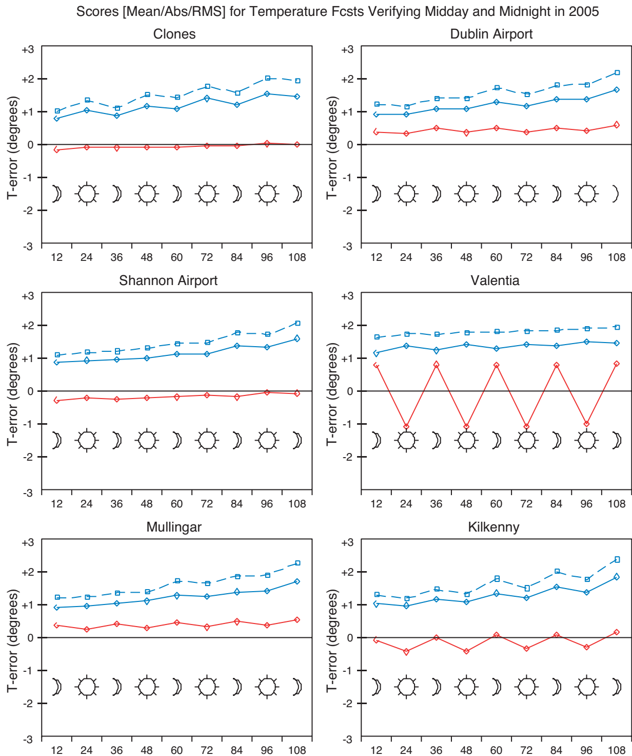
Fig. 7 Mean scores for ECMWF forecasts of 2-metre Temperature, in 2005, averaged over a year of data. The solid blue line is the mean absolute error, the dashed blue line the rms error and the red line the mean error or bias. It can be seen that the quality of the forecast decreases with the length of the forecast. The 'sun' and 'moon' symbols indicate forecasts verifying at midday and midnight, respectively. The length of the forecast [in hours] is indicated on the x-axis.
