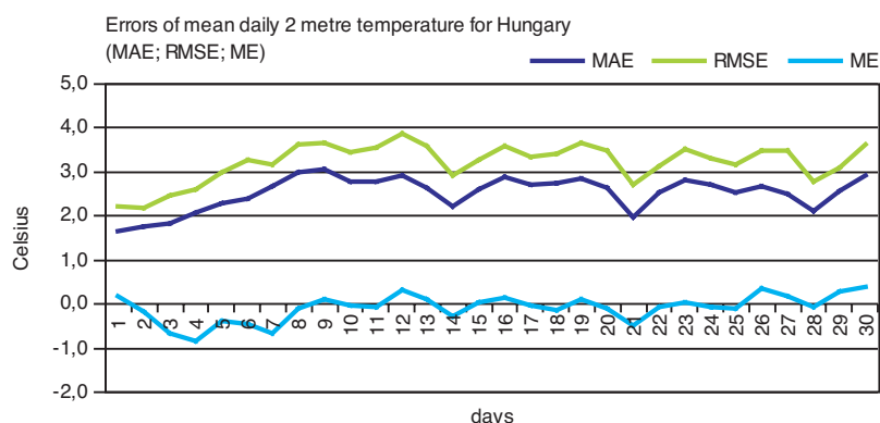
Fig. 17: Daily Mean Absolute Error (MAE), Root Mean Square Error (RMSE) and Mean Error (ME) of mean daily 2m temperature for Hungary (year 2005)
