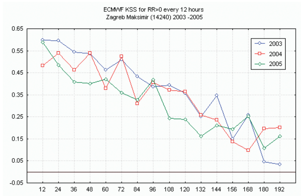
Fig. 4 The Hansen - Kuipers skill score for the 12-hour precipitation larger than 0 for Zagreb Maksimir
