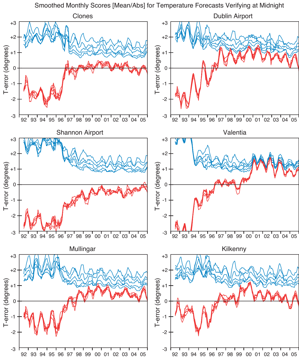
Fig. 4 Smoothed scores for the T+12, T+36, T+60, T+84, and T+108 ECMWF forecasts of 2-metre Temperature verifying at midnight. The lines were smoothed by taking a 5-month centred running mean. The blue lines show values of the monthly mean of the absolute error, the red lines values of the monthly mean of the mean error or bias. The top blue line corresponds to a T+106 forecast, the one below that to a T+84 forecast etc.
