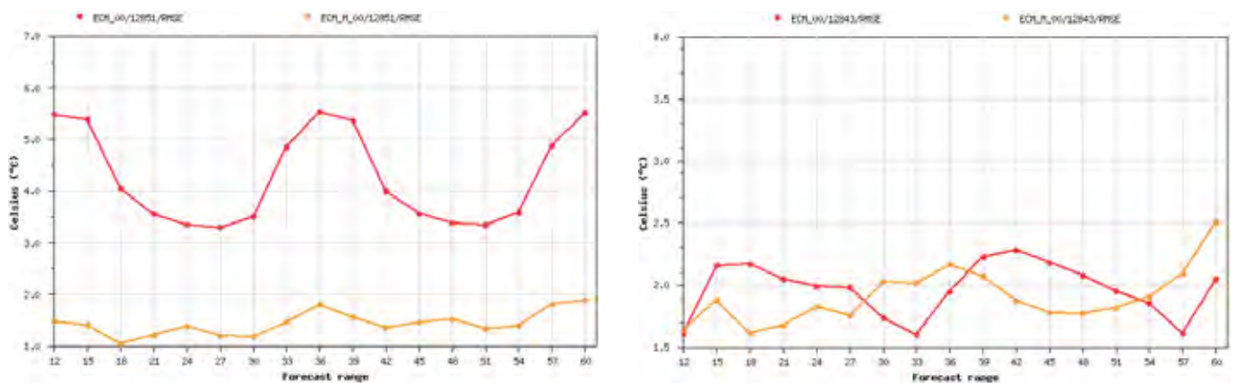
Fig. 11: The RMSE of the ECMWF 00 UTC 2m temperature forecasts before (red) and after (yellow) post-processing for the station Kékes-tető (1015 m, the highest point of Hungary, left panel) and for Budapest (right panel) in the period between 1st August 2005 and 31st January 2006. It is clear that the results over flat terrain are much less successful than that of stations with higher altitude.
