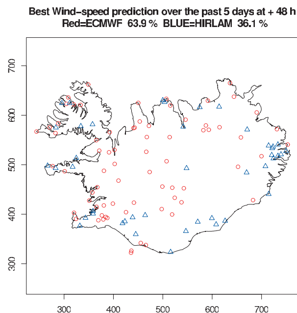
Fig. 5 Map of the best 10-metre wind-speed DMO forecasts over a 5-day period: (16/05/2006 - 20/05/2006). Red (blue) symbols indicate locations for which ECMWF (Hirnam) was better than Hirlam (ECMWF).
