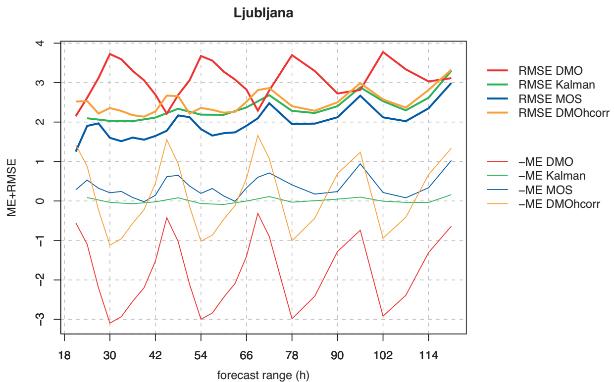
Fig. 2 Comparison of RMSE and ME for T2m forecast based on ECMWF deterministic forecast, 12 UTC: Direct Model Output (DMO), DMO with height correction (DMOhcorr), Kalman filtered values and Model Output Statistics (MOS) for T2m. Verification period is 1.1.2005 till 31.12.2005. Location: Ljubljana (14015)
