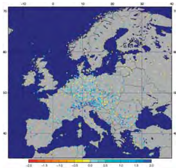
Fig. 10 The measure of success of the MOS technique over Europe. The blueish color indicates where the statistical post-processing improves the 2m temperature forecasts, while the “warm” colors indicates degradation. One can immediately spot improvements especially over mountainous areas (especially in the Alpine region).
