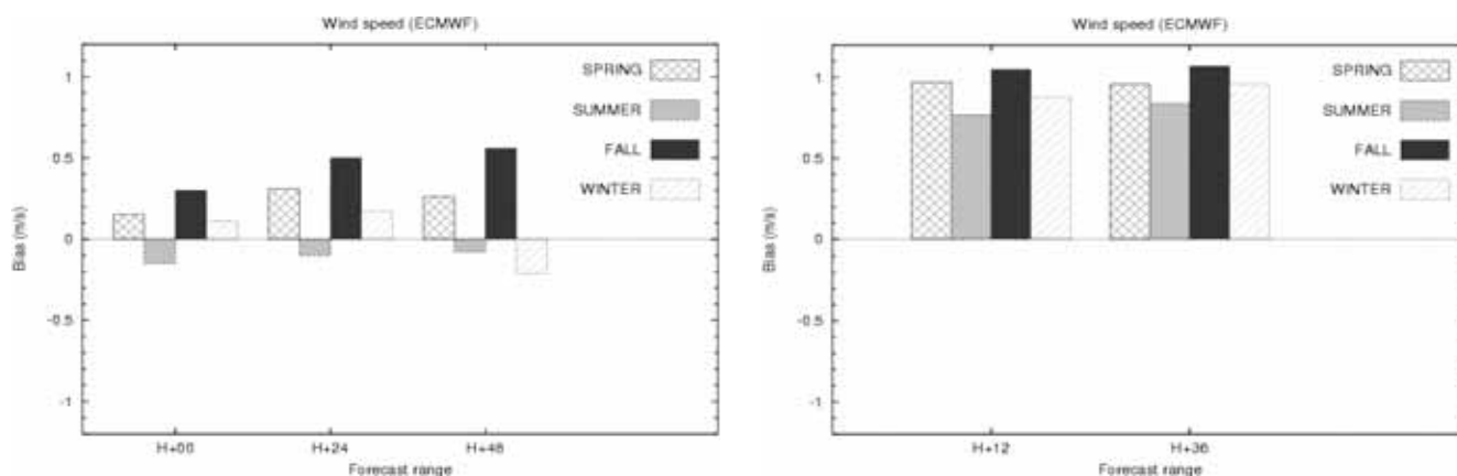
Fig. 12 Bias of 10m wind speed over Portugal as function of forecast range, for summer, spring, fall and winter seasons for 12 UTC (left) and for 00 UTC (right).
