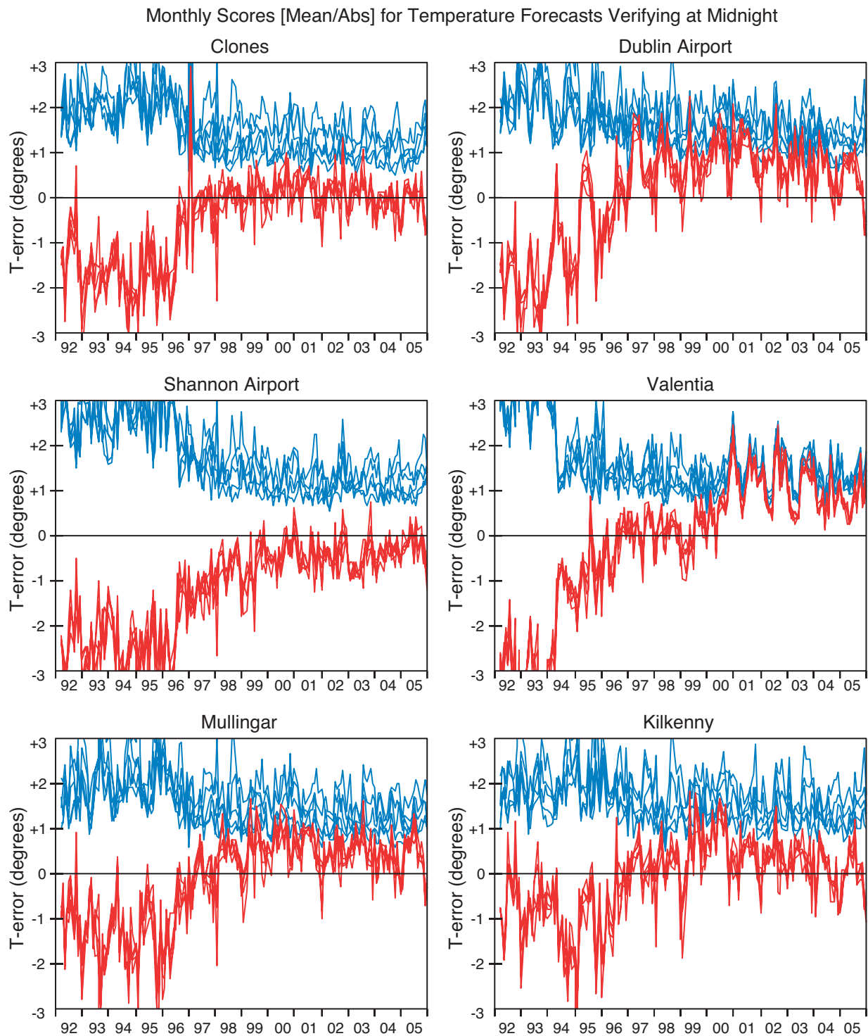
Fig. 2 Scores for the T+12, T+36, T+60, T+84, and T+108 ECMWF forecasts of 2-metre Temperature. Note that all these forecasts verify at midnight. The blue lines show values of the monthly mean of the absolute error, the red lines values of the monthly mean of the mean error or bias.
