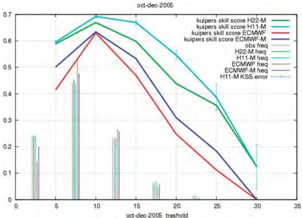
Fig. 12 KSS values for different thresholds for wind gust forecasts, The verification period is October to December 2005, for stations located south of 61 N. Red = ECMWF, light blue = MOS from HIRLAM with 11km resolution, green = MOS from HIRLAM with 22km resolution, dark blue = MOS from ECMWF. Observations are the maximum wind gust during a six hour period, centred around the forecast time. The observed relative frequencies in grey.
