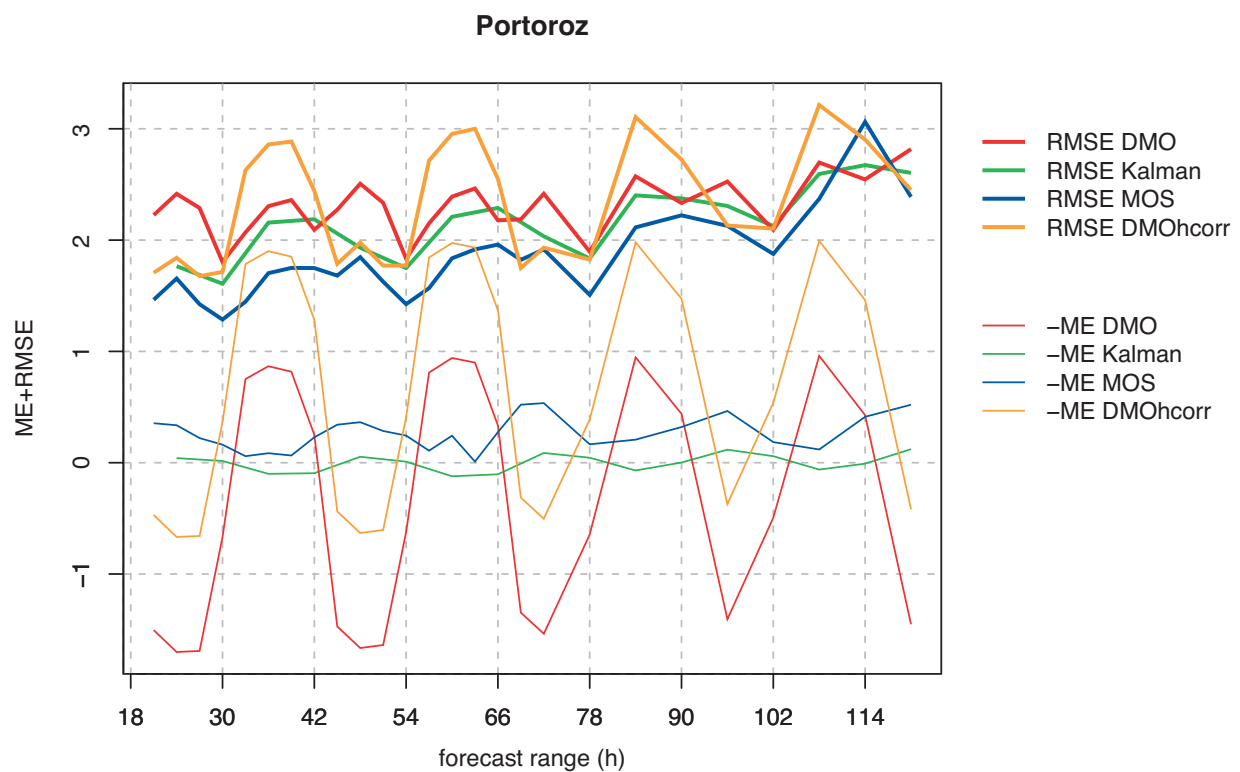
Fig. 4 Comparison of RMSE and ME for T2m forecast based on ECMWF deterministic forecast, 12 UTC: Direct Model Output (DMO), DMO with height correction (DMOhcorr), Kalman filtered values and Model Output Statistics (MOS) for T2m. Verification period is 1.1.2005 till 31.12.2005. Location: Portoroz (14105)
