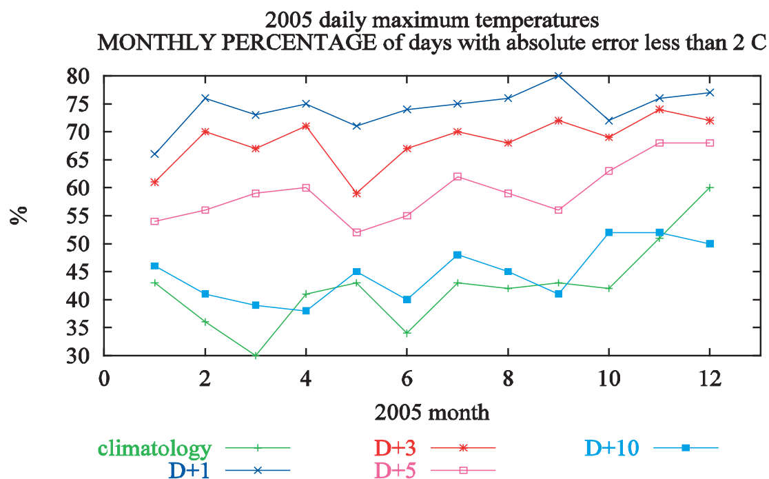
Fig. 2 Time series of percentage of correct maximum temperature forecasts (error less than 2°C) for different prediction ranges. The verification sample is composed by the forecasts made in 2005 for a set of 50 Spanish SYNOP stations.
