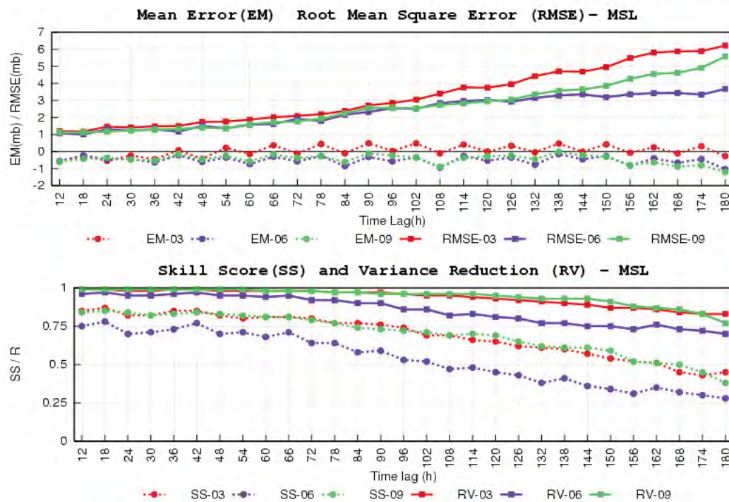
Fig. 6 Mean error (BIAS) and Root mean square error (RMSE) for Mean Sea Level Pressure (MSL) (upper panel) and Variance Reduction and MSE_SS (lower panel), averaged over 168 stations. Spring - Autumn 2005. (Red: Spring, Blue: Summer, Green: Autumn).
