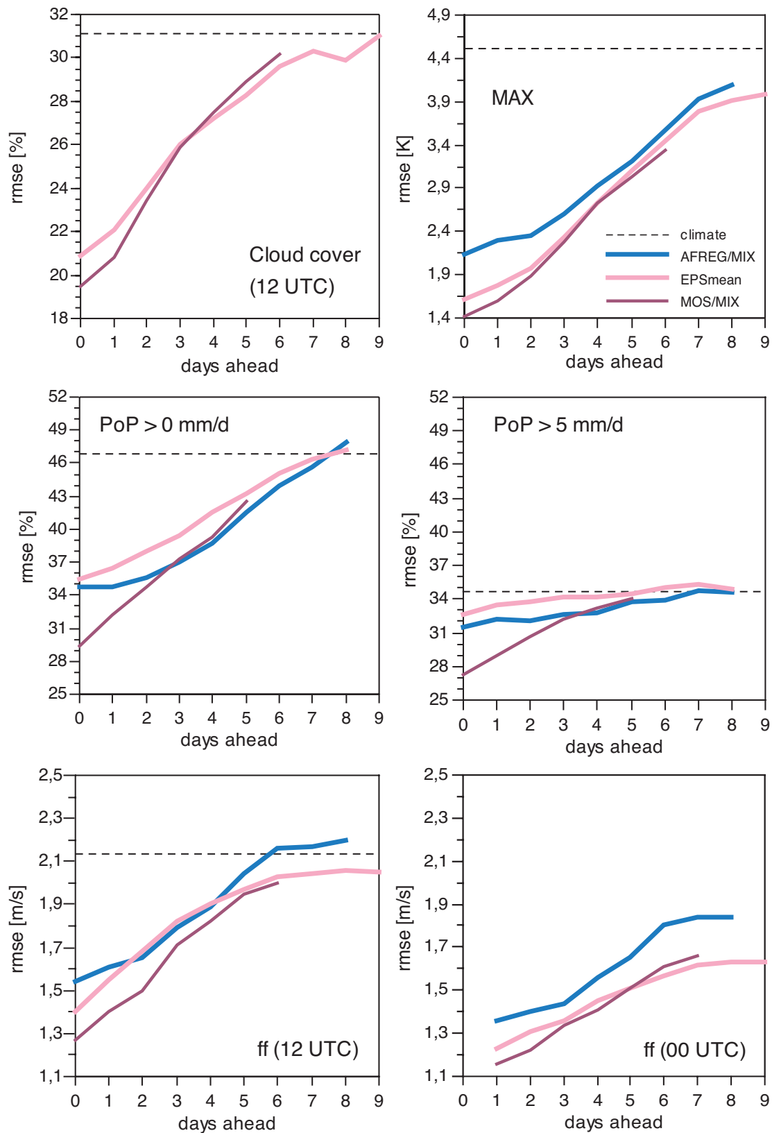
Fig. 6 DMO(EPSmean)+KAL (pink) versus AFREG-MIX (blue) and MOS/MIX (magenta), dotted line = rmse(climate).
