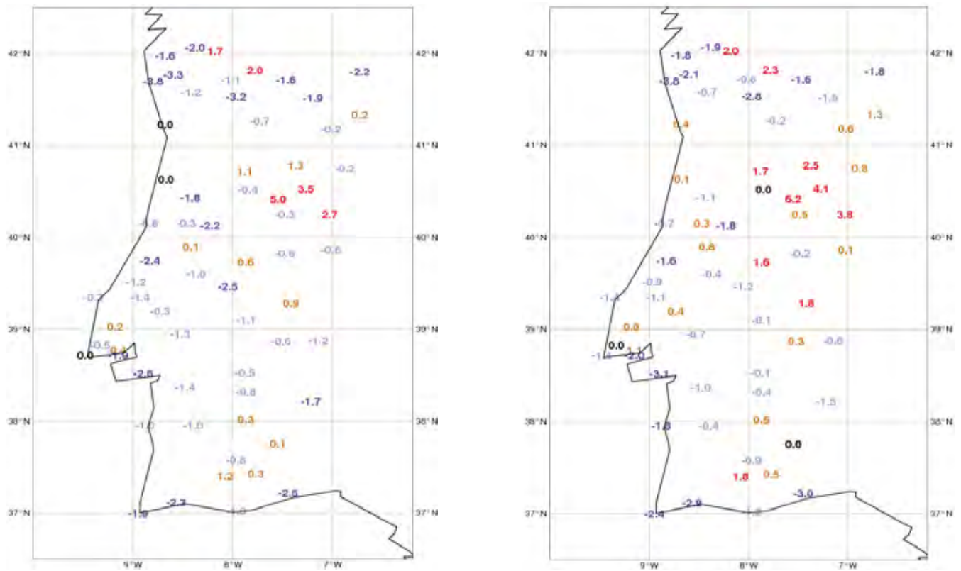
Fig. 2 Spatial distribution of 2m temperature bias over Portugal, for H+24 (valid at 12 UTC), for fall (left) and spring (right) seasons. Positive values are in red ( > 1.5^{\circ}\text{C} ) and orange ( \leq 1.5^{\circ}\text{C} ). Negative values are in blue ( < -1.5^{\circ}\text{C} ) and cyan ( \geq -1.5^{\circ}\text{C} ).
