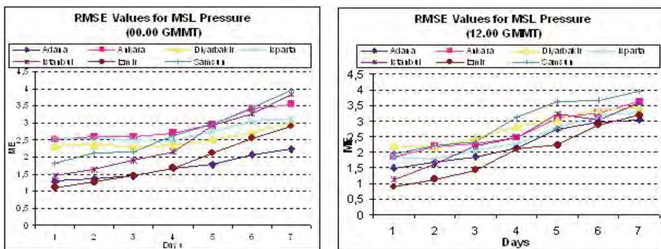
Fig. 2.1.1.10 Root Mean Square Errors of 00.00 and 12.00 UTC MSL Pressure forecasts as a function of forecast range for 7 Turkish radio-sonde stations
