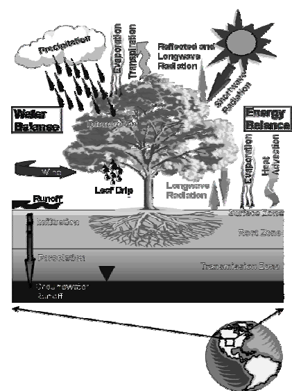
Fig 1: Land surface modeled processes.
