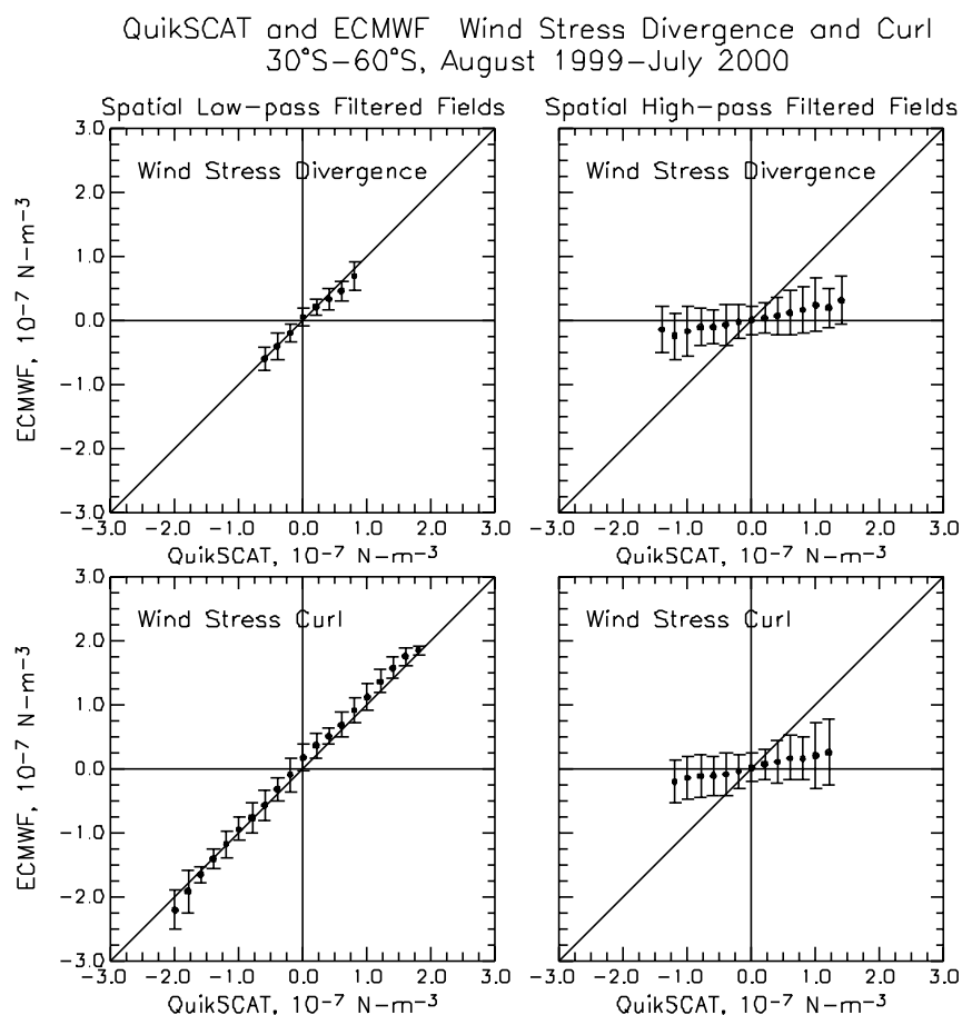
Figure 10 Binned scatter plots of ECMWF versus QuikSCAT wind stress divergence (top) and curl (bottom) on large (left) and on short (right) spatial scales. The filter cutoffs separating large and short scales are 30^\circ of longitude by 10^\circ of latitude. The error bars represent the standard deviations of the scatter within each bin.
