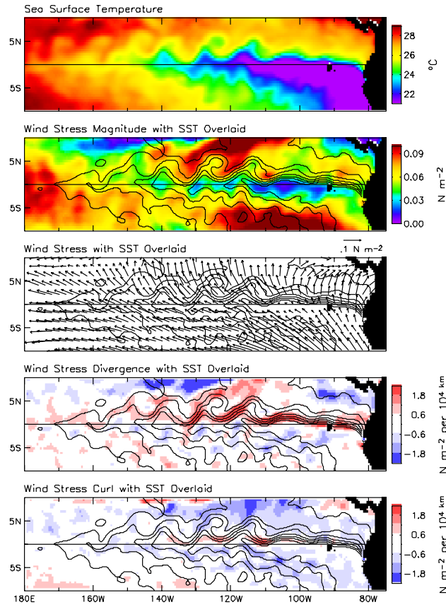
Figure 1 Maps for 4 September 1999 derived from QuikSCAT observations of wind stress and TMI observations of SST with spatial and temporal smoothing as described in the text. The SST in the top panel is overlaid with a contour interval of 1°C in the bottom four panels.
