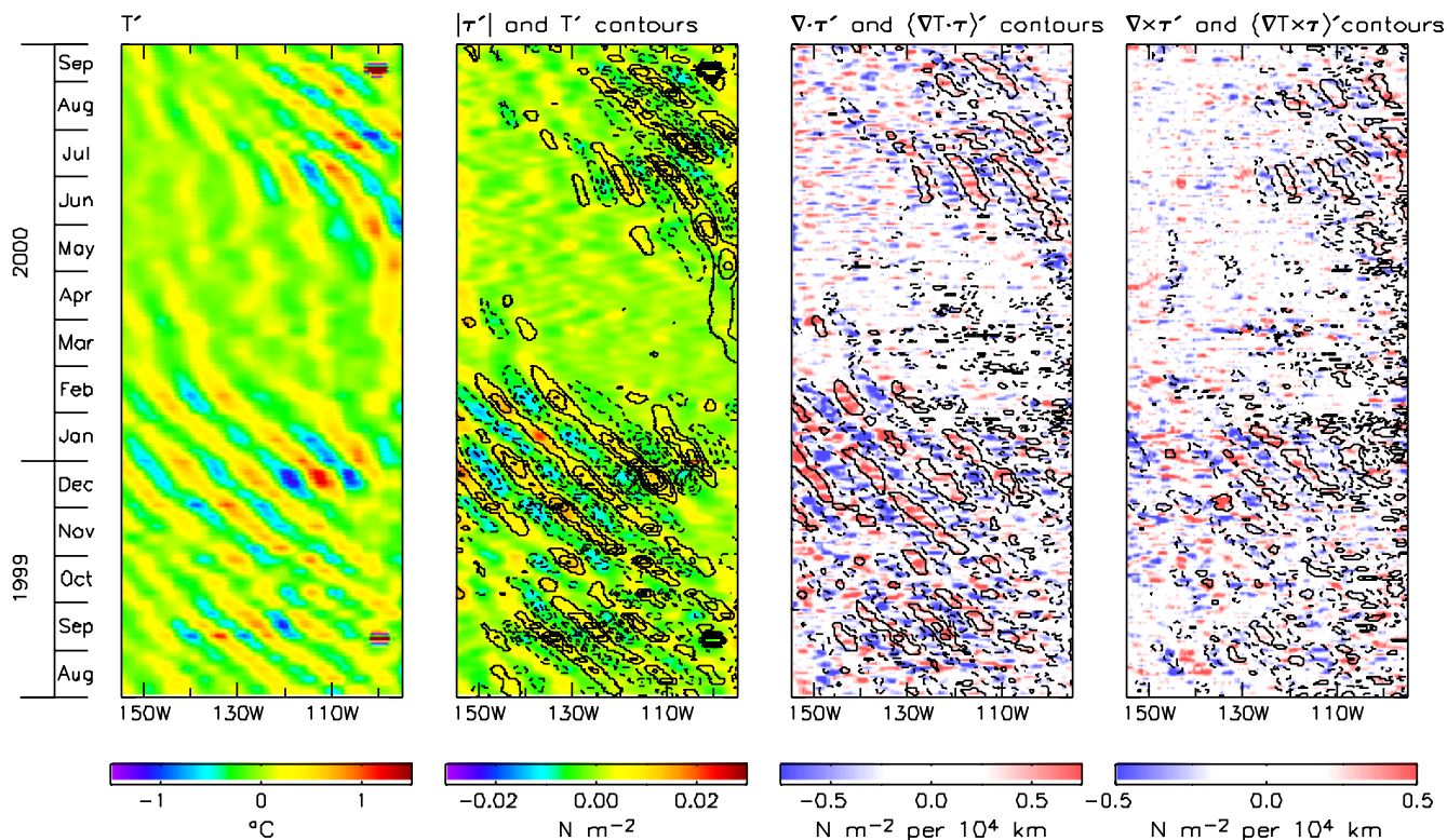
Figure 6 The same as Fig. 2, except from the ECMWF model wind stresses and Reynolds SST analyses along 1°N. The contour intervals are 0.25°C in the second panel and 0.25°C per 100 km in the right two panels. . Note that the color bars on the right two panels are different from the color bars on the right two panels of Fig. 2.
