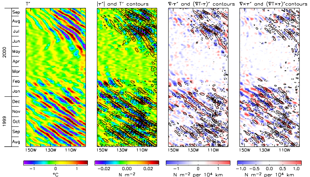
Figure 2 Time-longitude plots of QuikSCAT observations of wind stress and TMI observations of SST along 1°N showing westward propagation of SST, wind stress magnitude, wind stress divergence and wind stress curl (left to right) after zonally high-pass filtering to remove wavelengths longer than 20° of longitude. SST from the first panel is overlaid with a contour interval of 0.5°C in the second panel. The contours in the right two panels are the downwind and crosswind SST gradients, respectively, with contour intervals of 0.4°C per 100 km. The zero contours have been omitted from the three right panels for clarity.
