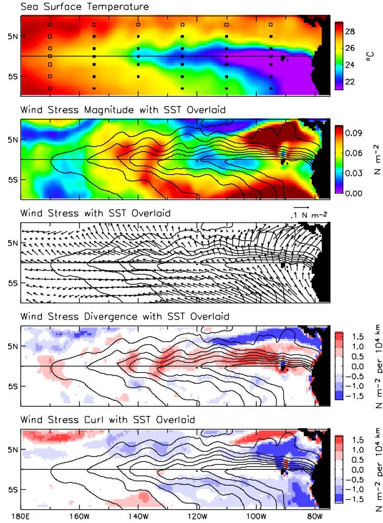
Figure 5 The same as Fig. 1, except derived from the ECMWF model wind stresses and Reynolds SST analyses. Note that the color bars on the bottom two panels are different from the color bars on the bottom two panels of Fig. 1.
