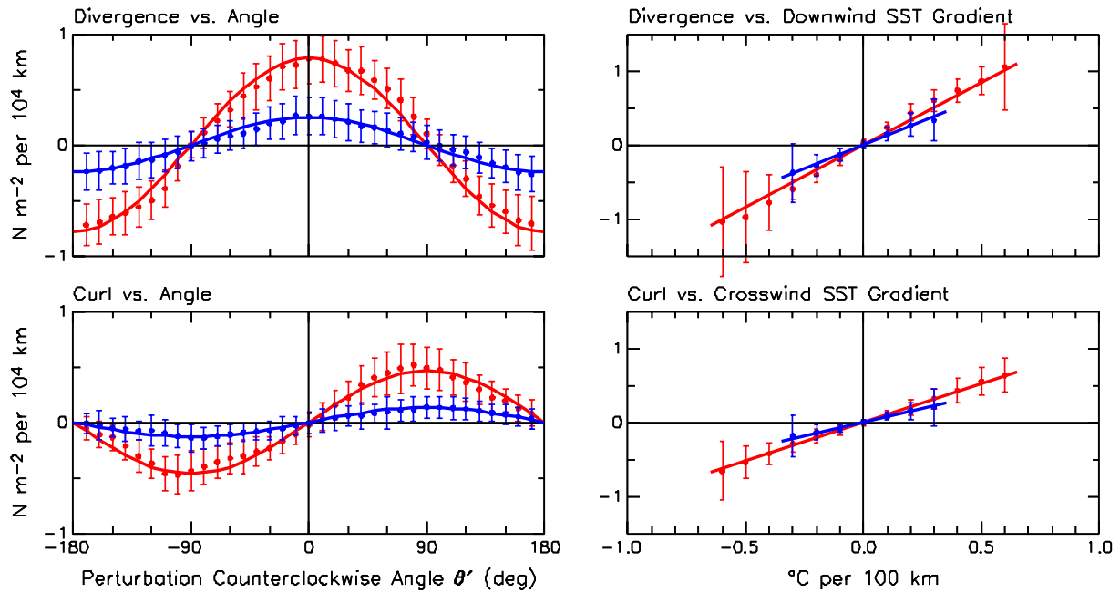
Figure 3 Left: Binned scatterplots of the angular dependencies of zonally high-pass filtered wind stress divergence (top) and curl (bottom) on the angle between the SST gradient vector and the wind direction in the region 150°–100°W and 1°S to 3°N. Right: Binned scatterplots of the relationships between zonally high-pass filtered wind stress divergence and the downwind gradient of SST (top) and between the zonally high-pass filtered wind stress curl and the crosswind gradient of SST (bottom). The error bars in all plots represent the standard deviations of the scatter within each bin. The red lines are the results obtained from the QuikSCAT and TMI observations and the blue lines are the results obtained from the ECMWF model wind stresses and Reynolds SST analyses.
