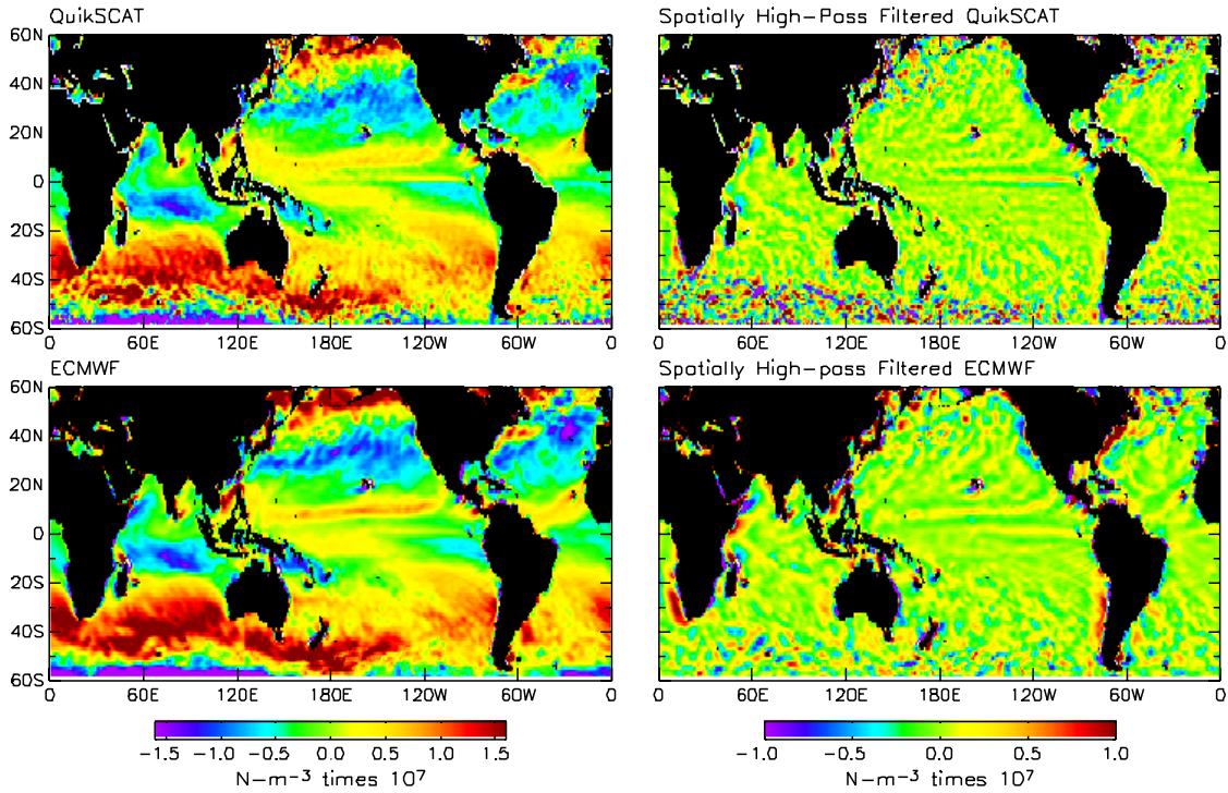
Figure 8 The same as Fig. 7, except for the wind stress curl.
