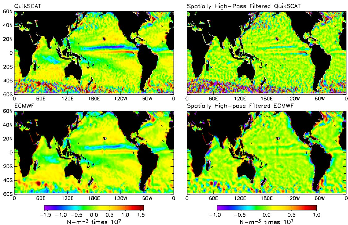
Figure 7 Average maps of the wind stress divergence over the 12-month period August 1999 through July 2000 derived from QuikSCAT observations (top) and the ECMWF model (bottom). The right panels show the spatially high-pass filtered fields obtained by removing variability with scales longer than 30° of longitude by 10° of latitude.
