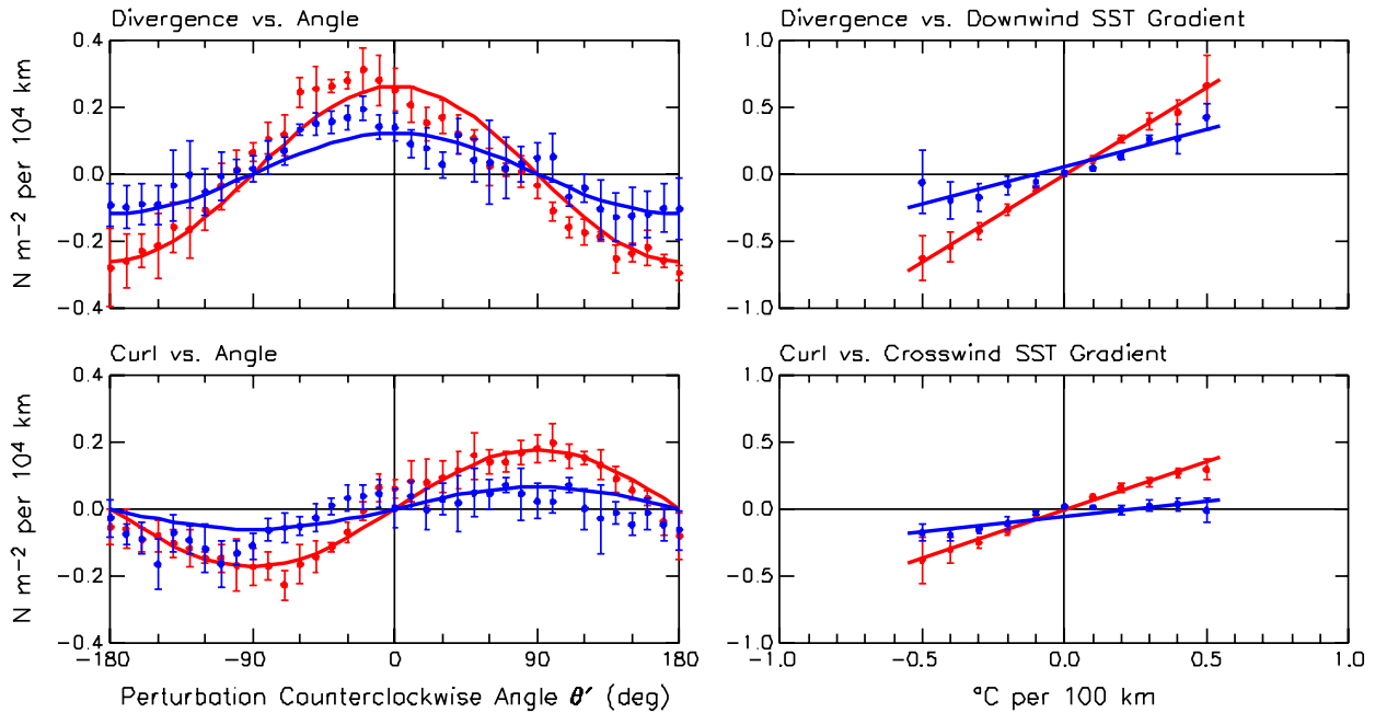
Figure 9 The same as Fig. 3, except for the latitude band 30°S to 60°S. Because TMI SST observations are not available south of 38°S, the QuikSCAT data are compared here with the Reynolds SST analyses.
