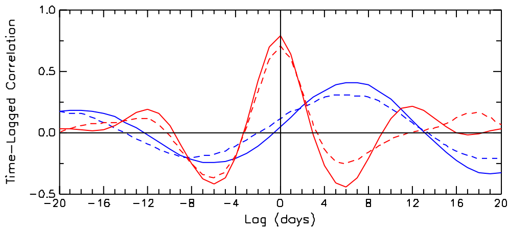
Figure 4 Lagged cross correlations between the wind stress divergence and the downwind gradient of SST (solid lines) and between the wind stress curl and the crosswind gradient of SST (dashed lines). Positive lags correspond to SST leading the wind stress. The red lines are the results obtained from the QuikSCAT and TMI observations and the blue lines are the results obtained from the ECMWF model wind stresses and Reynolds SST analyses.
