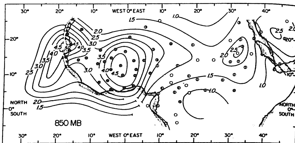
Fig. 15 Amplitude of meridional wind oscillation ( \text{m s}^{-1} ) in the frequency band 0.2-0.4 cpd at 850 mb.
