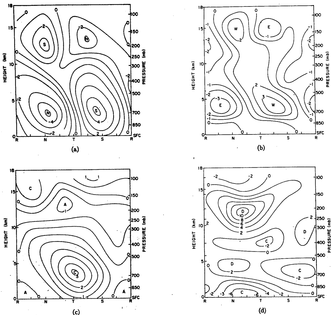
Fig. 13 Vertical cross sections along reference latitude. (a) Meridional wind deviation ( \text{m s}^{-1} ); (b) zonal wind deviation ( \text{m s}^{-1} ); (c) vorticity ( 10^{-5} \text{s}^{-1} ); (d) divergence ( 10^{-6} \text{s}^{-1} ). R, N, T, S refer to ridge, north wind, trough, south wind sectors of the wave, respectively.
