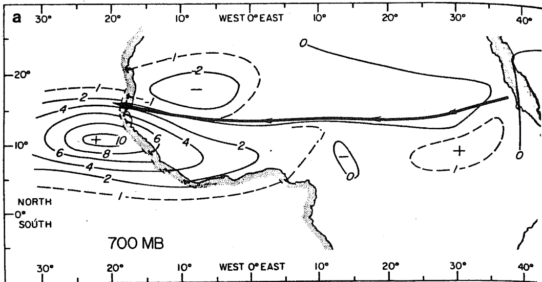
Fig. 16 Northward flux of zonal momentum ( \overline{uv} ) at 700 mb in 0.2 - 0.4 cpd frequency band. Units: \text{m}^2\text{s}^{-2} .
