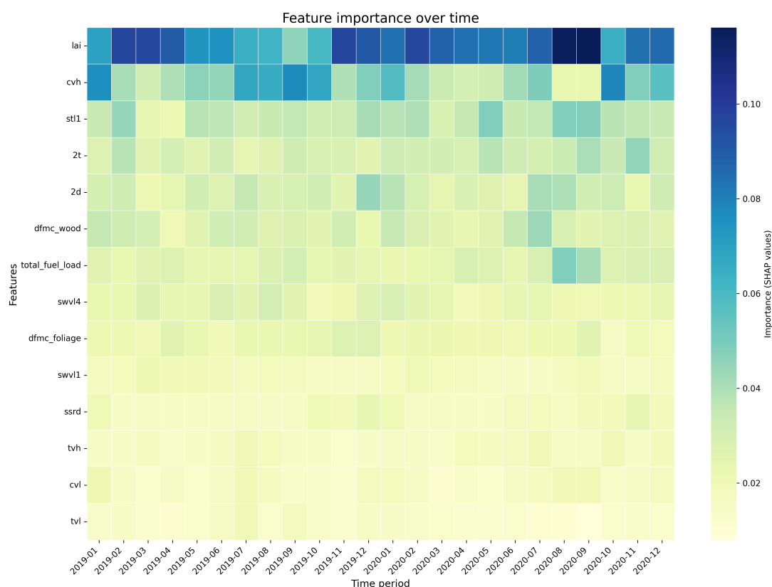
Figure A.14: Feature importance over time derived using SHAP values for an XGBoost model built separately for each month to predict C-VOD. The analysis spans the training period from 2019 to 2020, using monthly satellite observations. The heatmap highlights seasonal patterns. Darker blue shades represent features with greater influence on model predictions.
