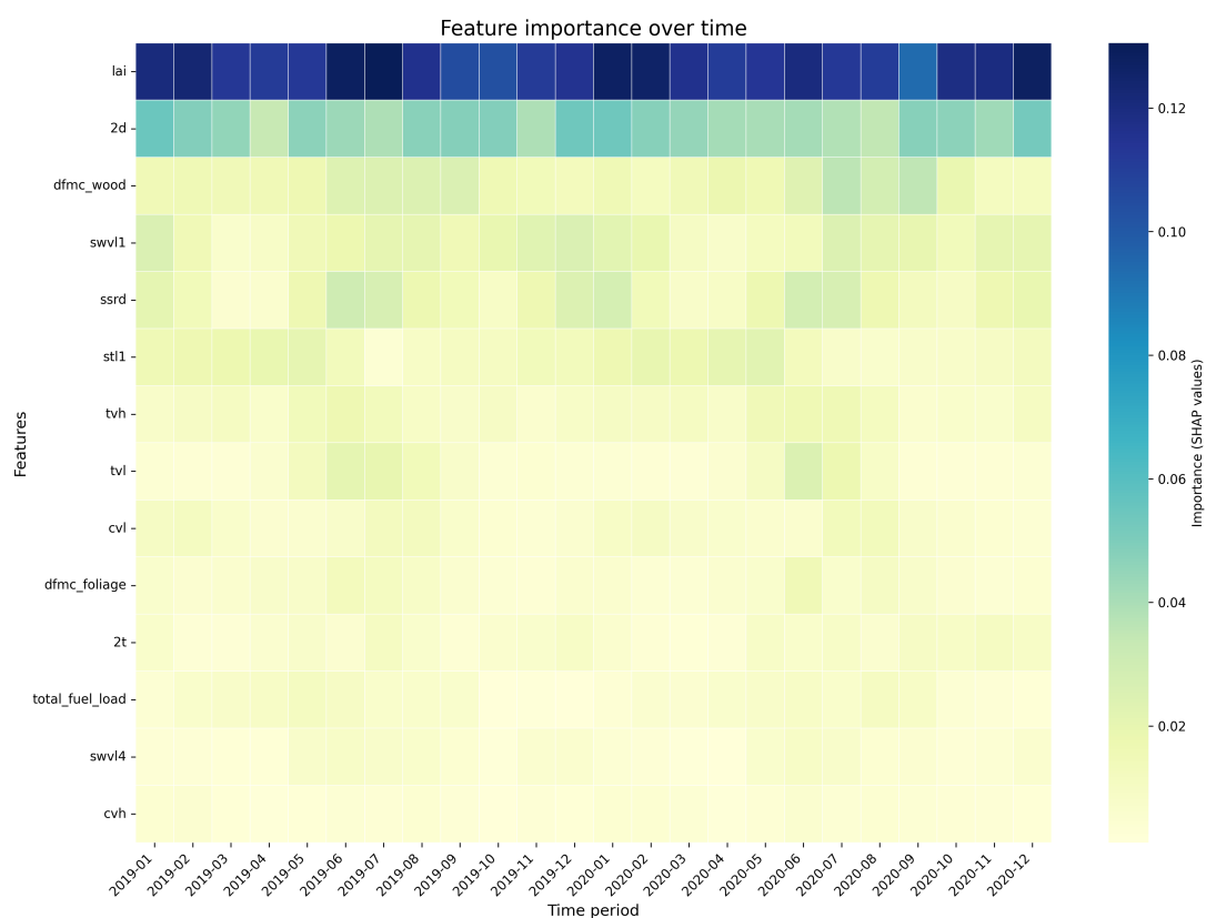
Figure A.13: Feature importance over time derived using SHAP values for an XGBoost model built separately for each month to predict SIF. The analysis spans the training period from 2019 to 2020, using monthly satellite observations. The heatmap highlights seasonal patterns. Darker blue shades represent features with greater influence on model predictions.
