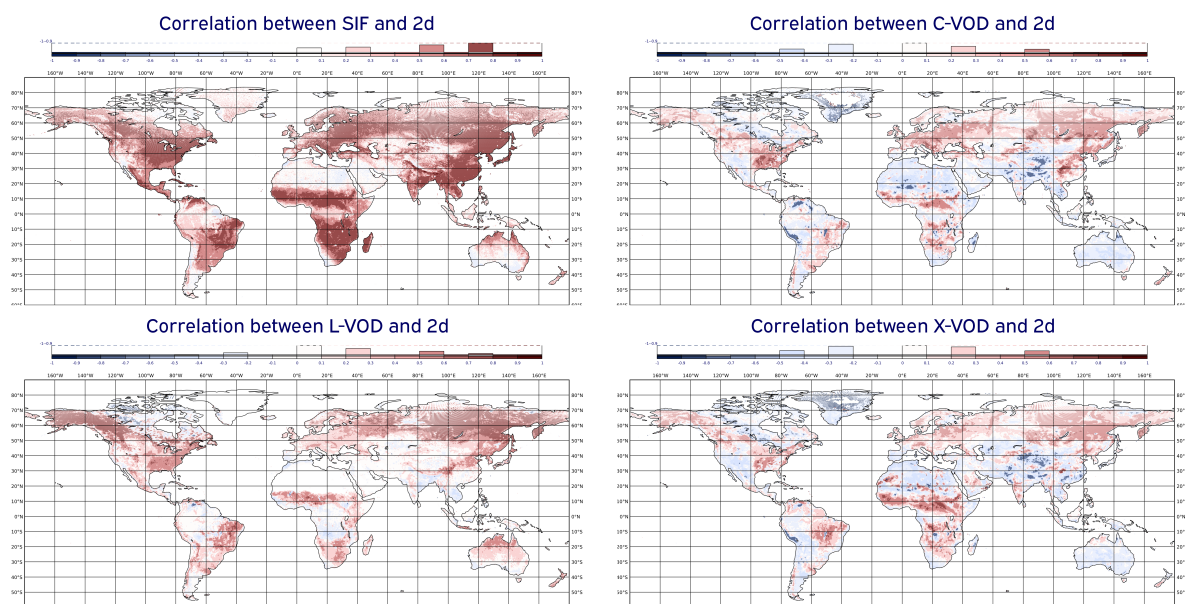
Figure 5: Spatial map of temporal correlation between 2-metre dewpoint temperature (2d) and satellite observations over the period 2019–2021. The top-left panel shows the correlation with SIF, the top-right panel with C-VOD, the bottom-left panel with L-VOD, and the bottom-right panel with X-VOD. Red shading indicates positive correlations, while blue shading indicates negative correlations.
